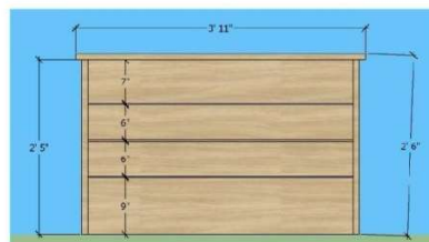
OFFICE DESK MEDIUM FRONT ELEVATION
