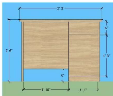
COMPUTER DESK BACK ELEVATION
