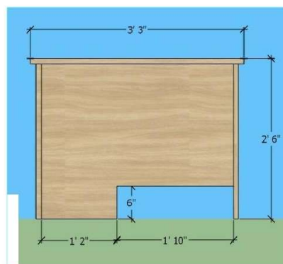
COMPUTER DESK FTRN ELEVATION
