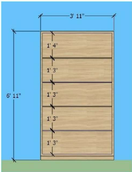
OPEN RACK FOR OFFICE FACULTY FRONT ELEVATION
