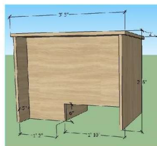
COMPUTER DESK ISO VIEW
