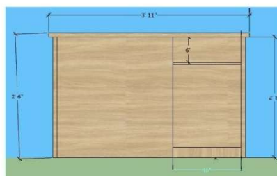
OFFICE DESK MEDIUM BACK ELEVATION
