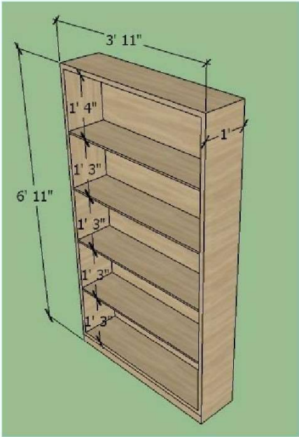
OPEN RACK FOR OFFICE FACULTY ISO VIEW
