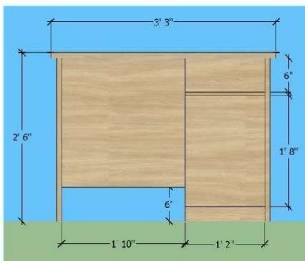
COMPUTER DESK BACK ELEVATION
