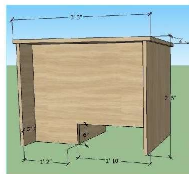
COMPUTER DESK ISO VIEW
