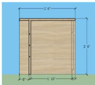
OFFICE DESK MEDIUM SECTION
