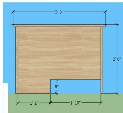
COMPUTER DESK FTRN ELEVATION
