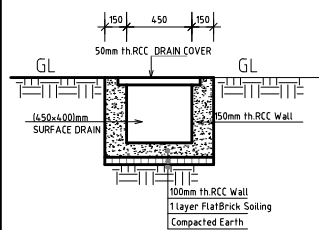
PRIMARY DRAIN
