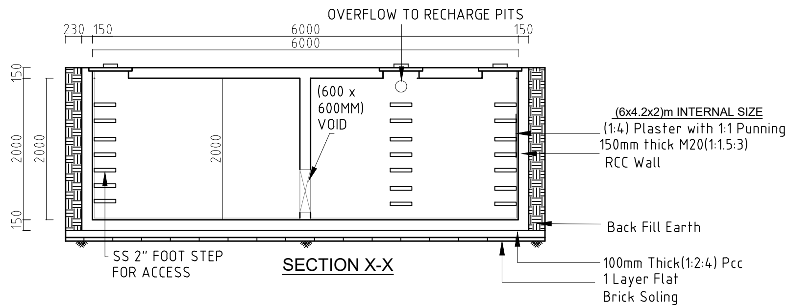
RAINWATER COLLECTION TANK-2 (RWCT-2) DETAILS
