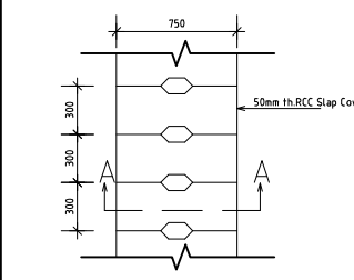
Plan Of Drain COVER
