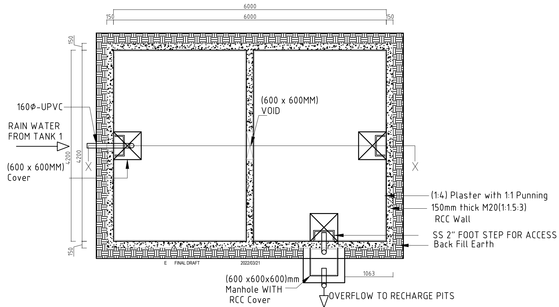
SECTIONAL PLAN
