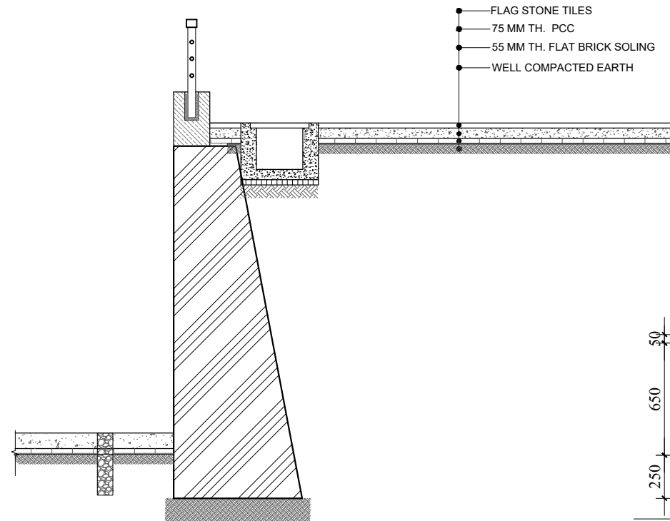
DETAILS D
