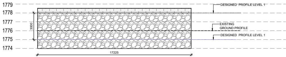
SECTION AT 3
