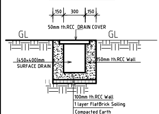
SECONDARY DRAIN
