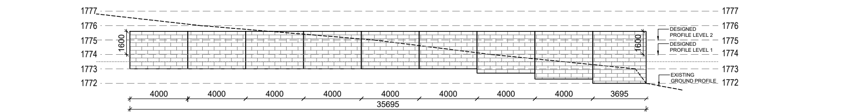
SECTION AT 15
