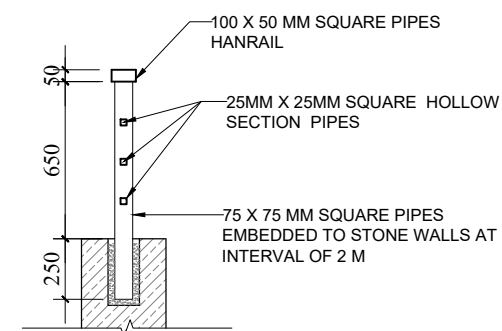
RAILING DETAILS
