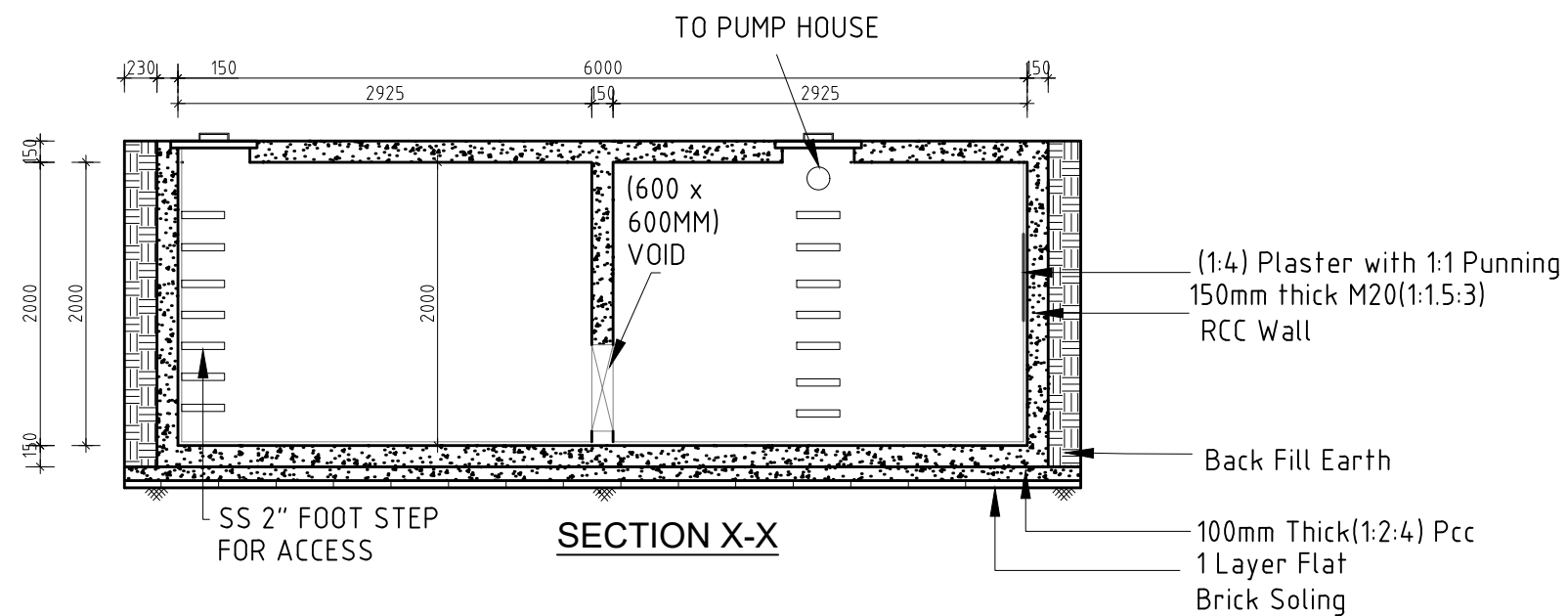
FIREFIGHTING WATER TANK (6X4.2X2)m Internal DETAILS
