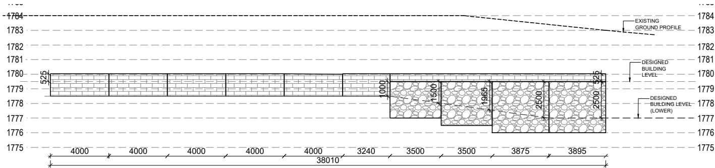
SECTION AT 8
