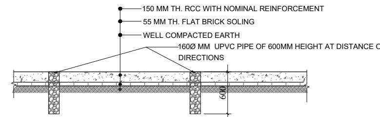
DETAILS C
