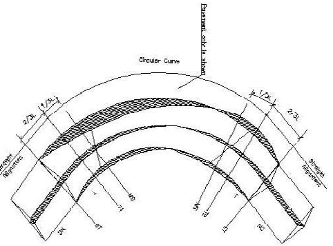
Typical Super-elevation
