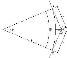
Circular Curve For Horizontal Alignment
